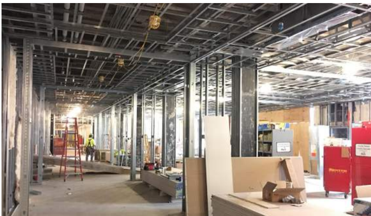
Ceiling & Wall Framing Installation Area G 3rd Floor
